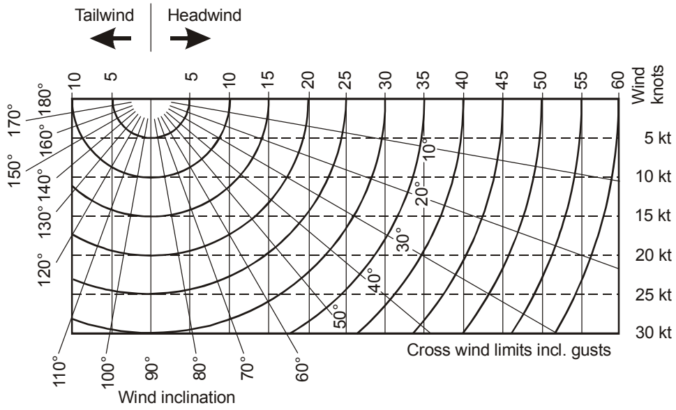
Figure A6-5. Typical wind limit diagram
