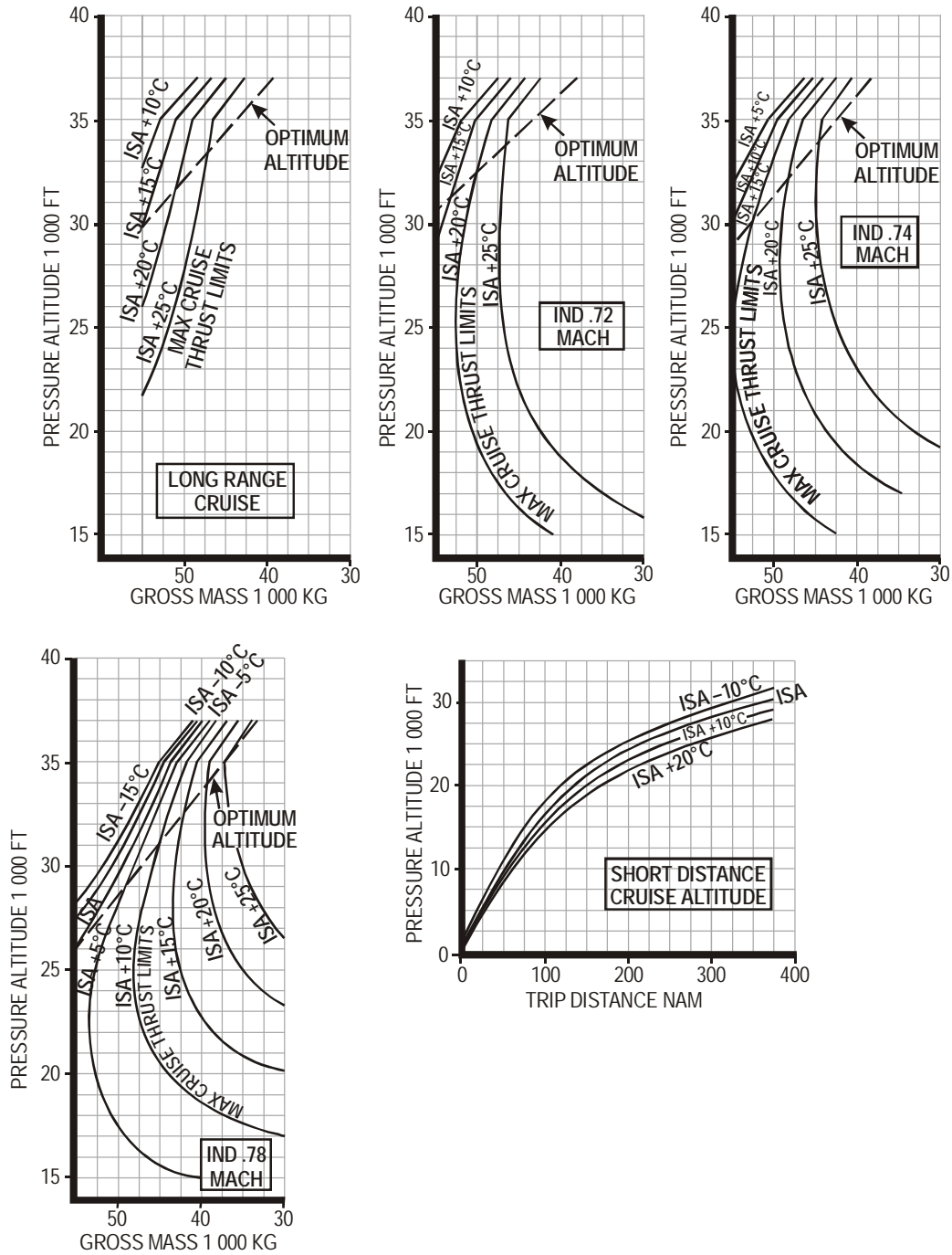
Figure A6-3. Optimum flight level (for B737) as a function of take-off mass and temperature deviation from standard
